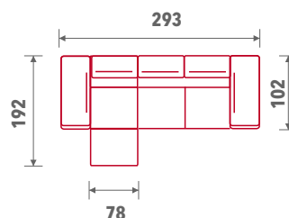
Sastav 13 (63F*+46+28F*+64F*)
