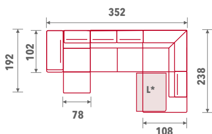
Sastav 09 (63F*+46+28F*+50+41L*)
